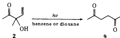
Scheme I. Direct Photolysis of 3-Hydroxy-3-methylpent-4-en-2-one
